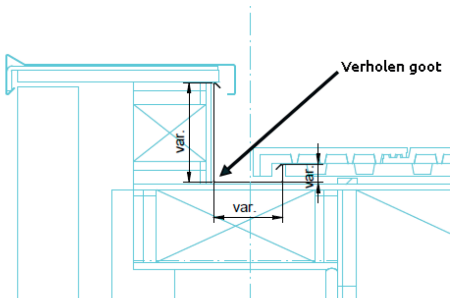
Variabele goot
